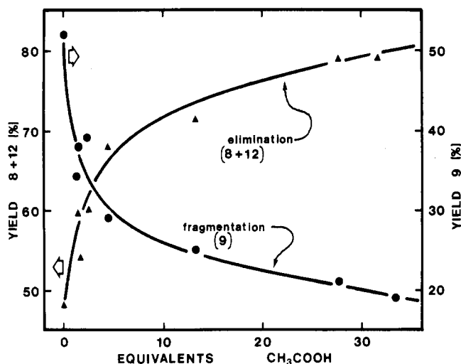
Figure 1. Correlation of elimination (▲) and fragmentation (●) yields with equivalents of acetic acid added to tetramethylammonium acetate (0.014 M) as catalyst.
